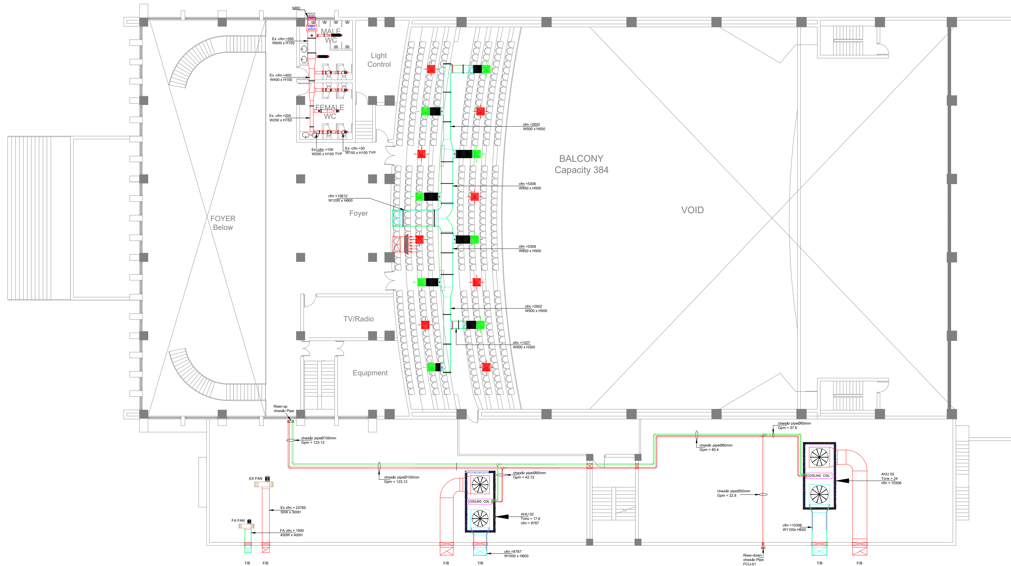
SECOND FLOOR PLAN (lvl.+11000) Area: 1919 Sq.m Scale= 1:250
